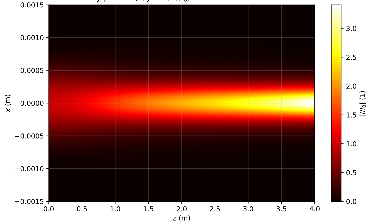
Intensity profile I(x, y = 0, z)/I_0 , P_{in}=1.0P_{cr} , artificial time
